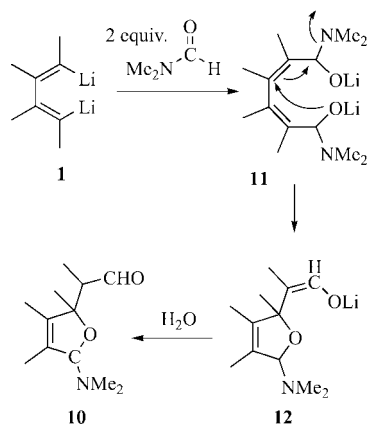
Scheme 6. Proposed reaction mechanism for the formation of 10 .
